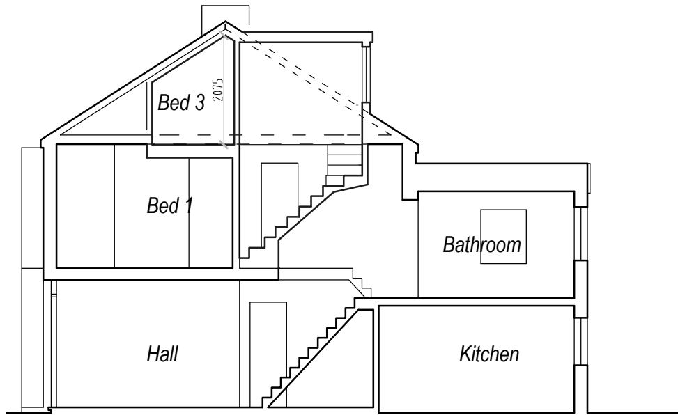
Section A-A @ 1:100
