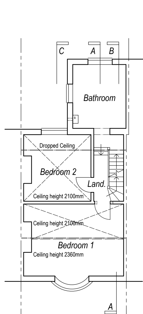
First Floor Plan @ 1:100
