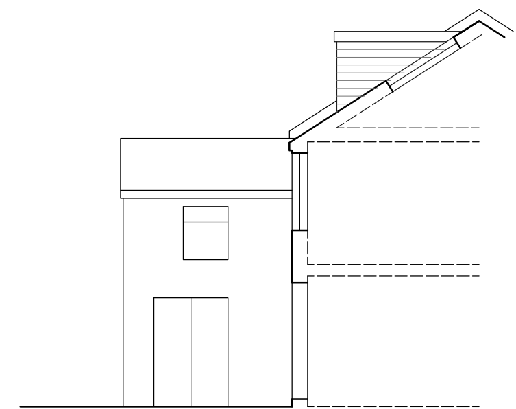
Side (East) Elevation/Section C-C @ 1:100
