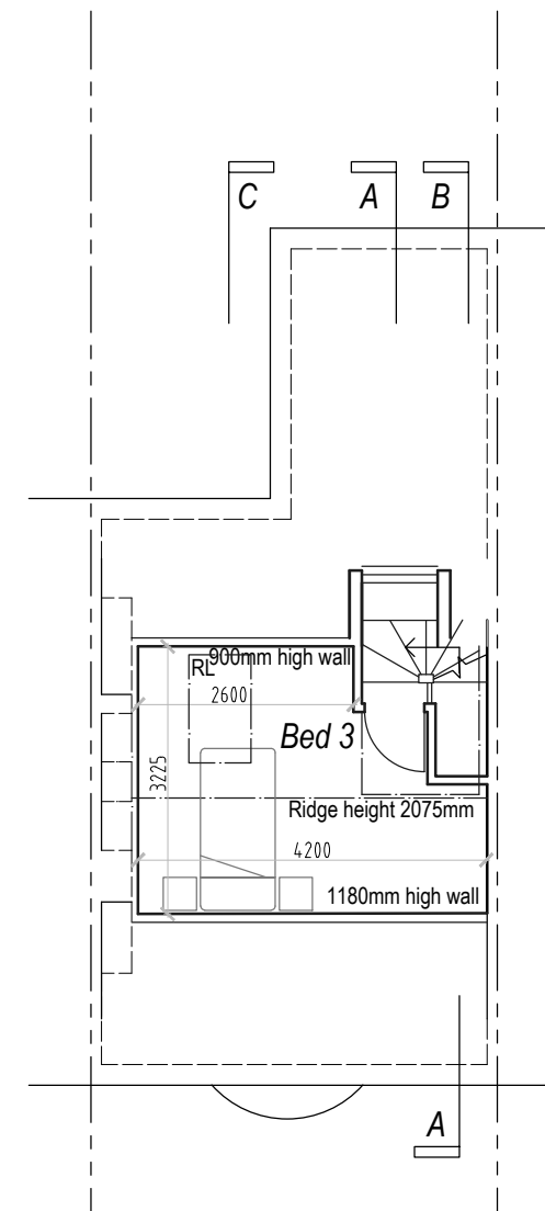
Loft Plan @ 1:100
