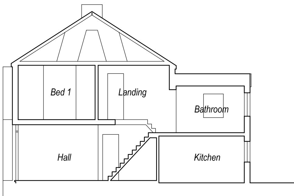
Section A-A @ 1:100
