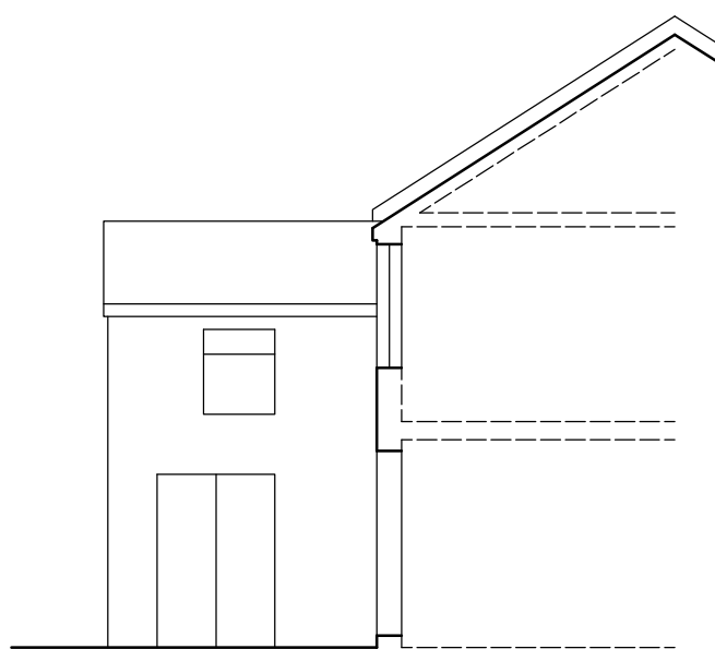
Side (East) Elevation/Section C-C @ 1:100
