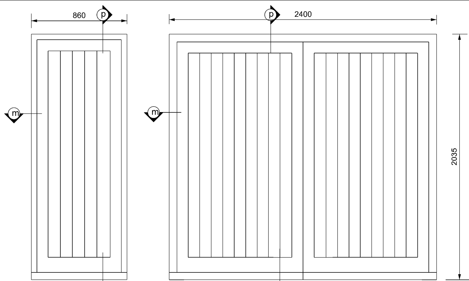
DOOR D1 1 NO. THUS: SOUTH ELEVATION Hardwood framed & boarded door
