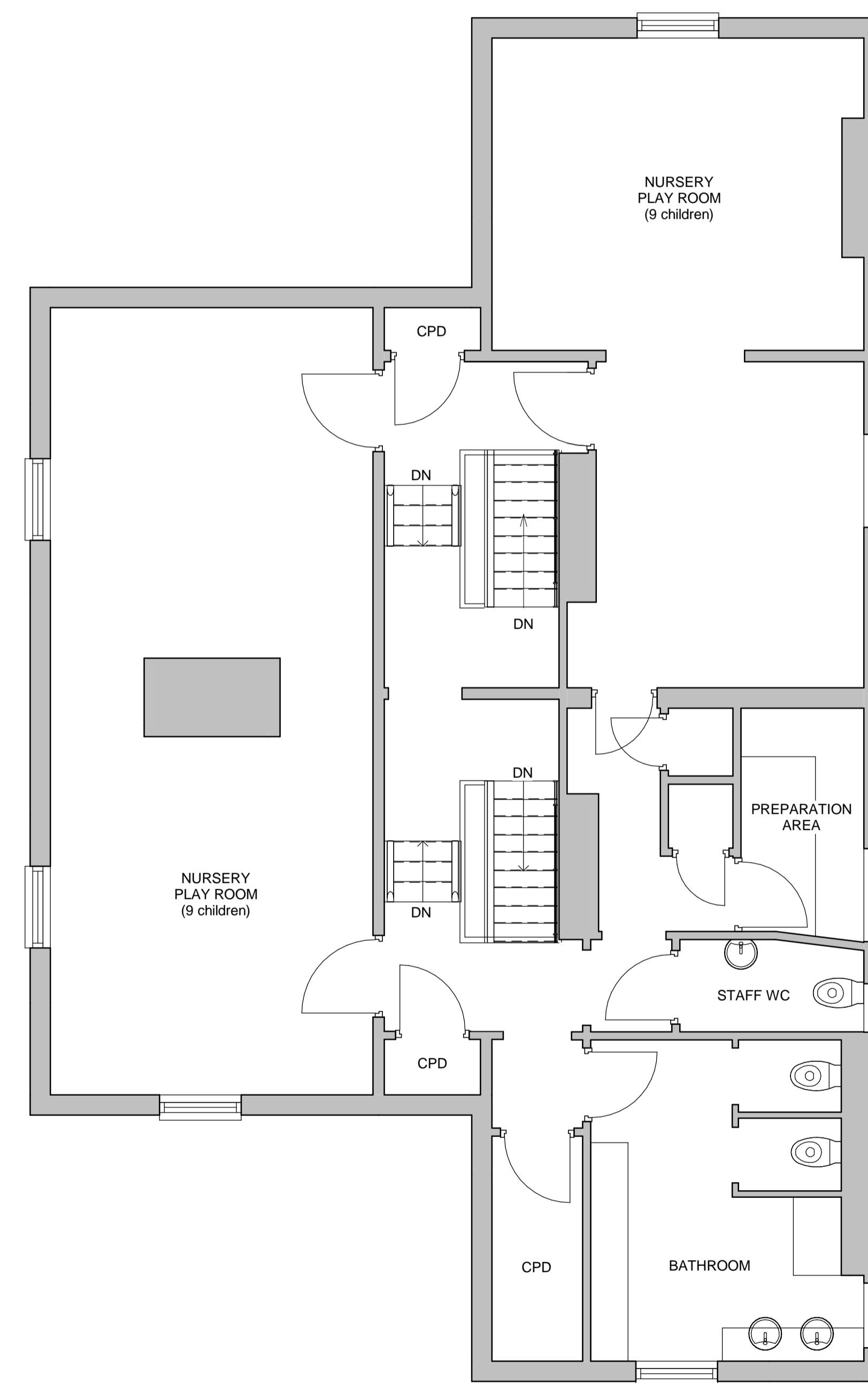
2 First Floor 1 : 50
