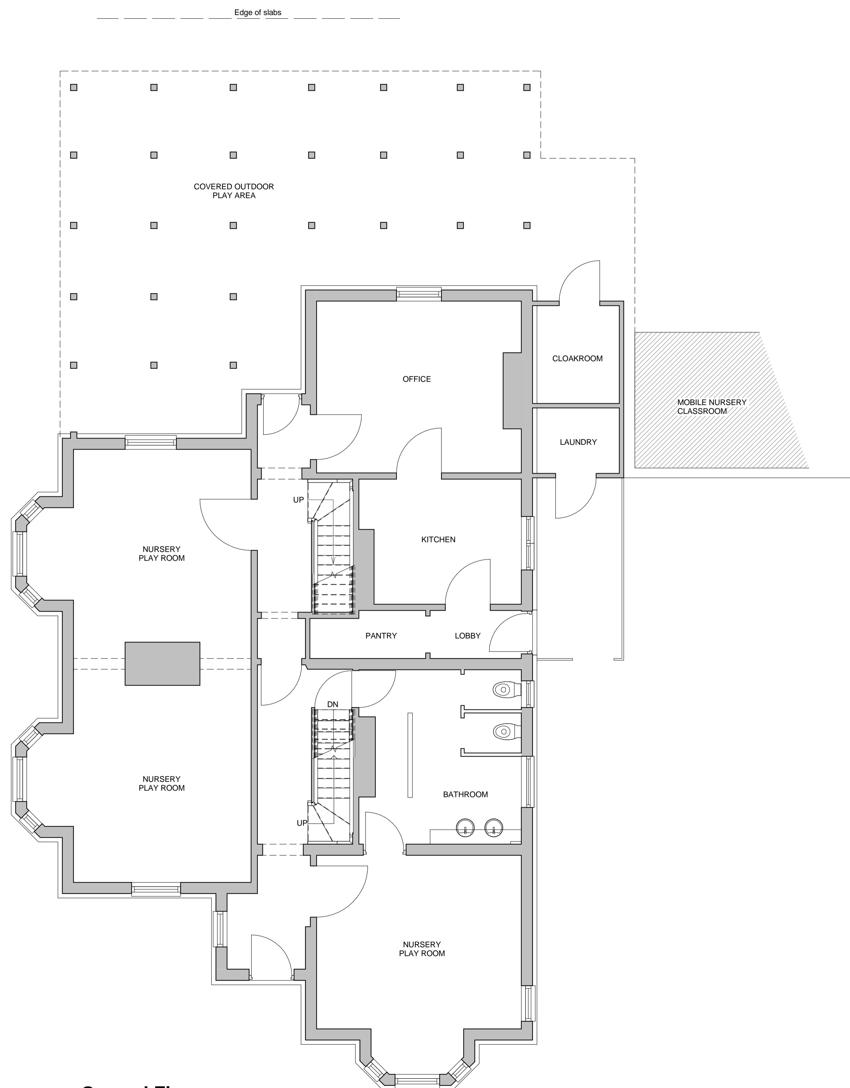
1 Ground Floor 1 : 50
