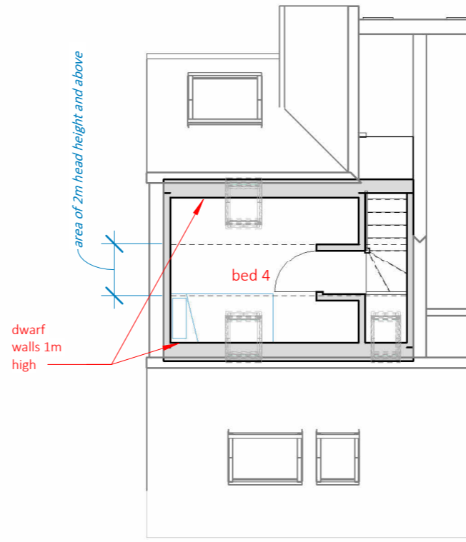
3 P03 P5.0 Second Floor as proposed 1 : 100
