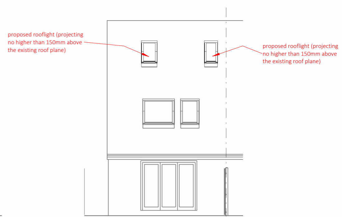
7 P03 south elevation - proposed 1 : 100
