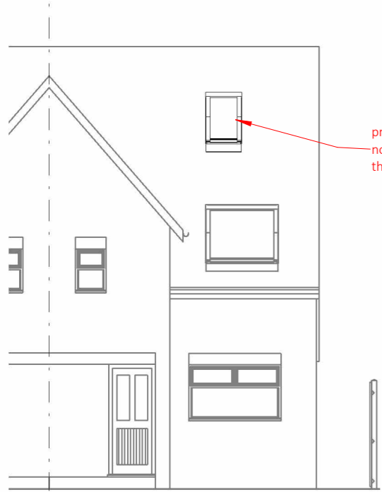
5 P03 north elevation - proposed 1 : 100
