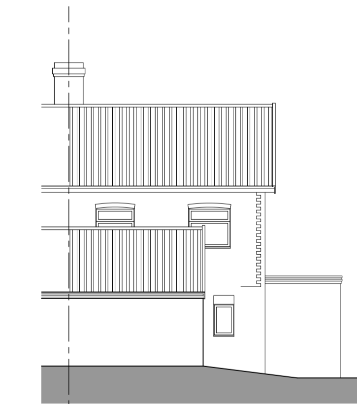
rear elevation (north east)
