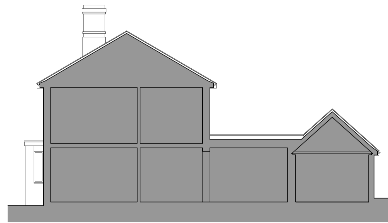
section elevation a (south east)
