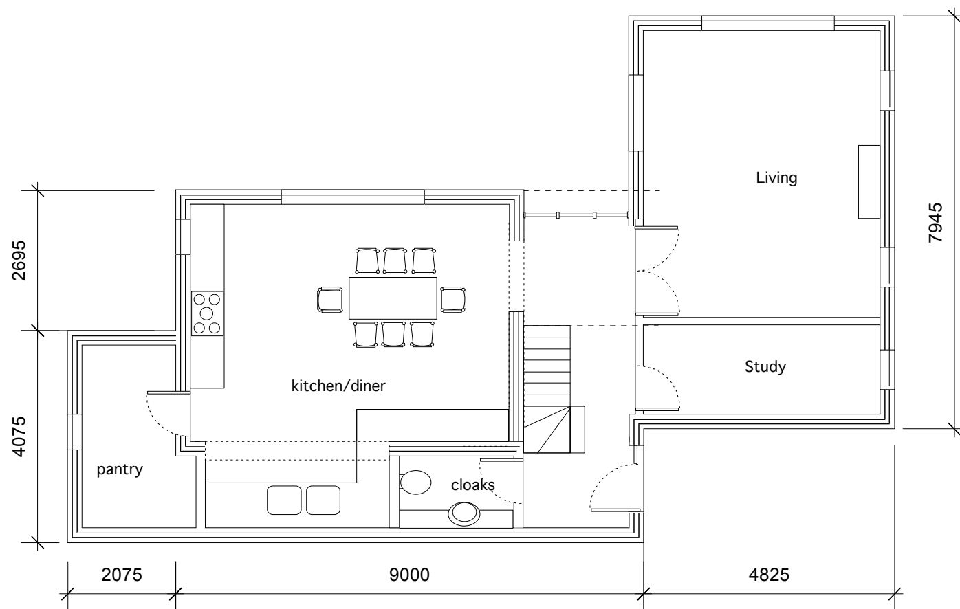
EXISTING GROUND FLOOR PLANS
