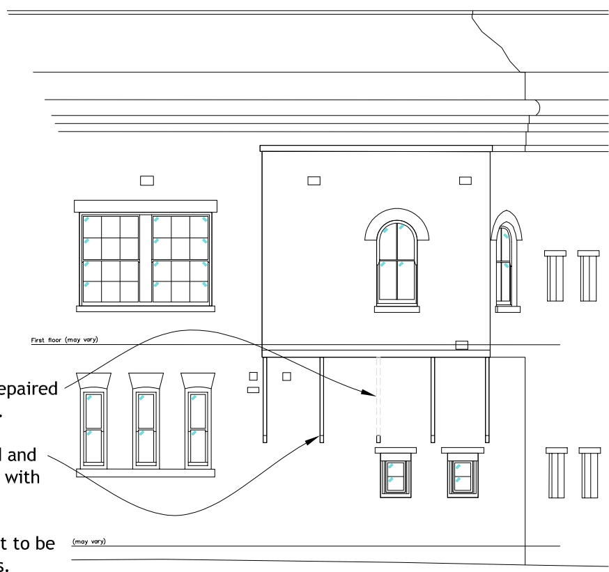
NORTH-WEST ELEVATION
