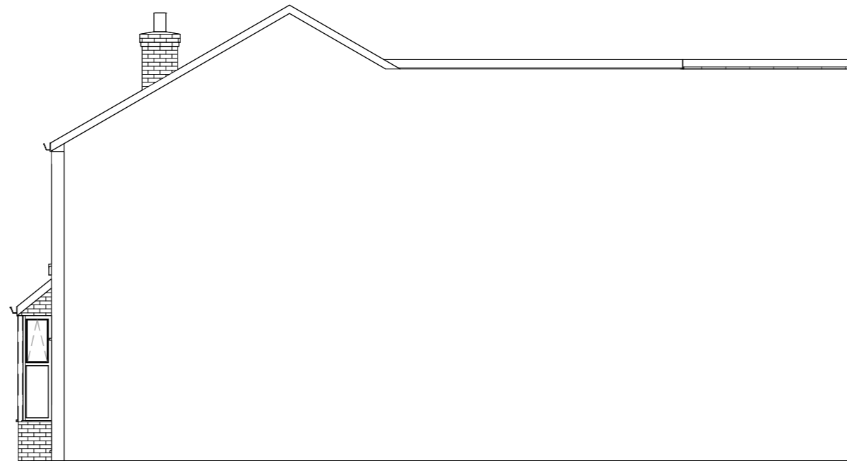
5 side Elevation 1 : 100
