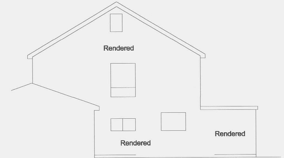
PART RIGHT FLANK ELEVATION AS EXISTING
