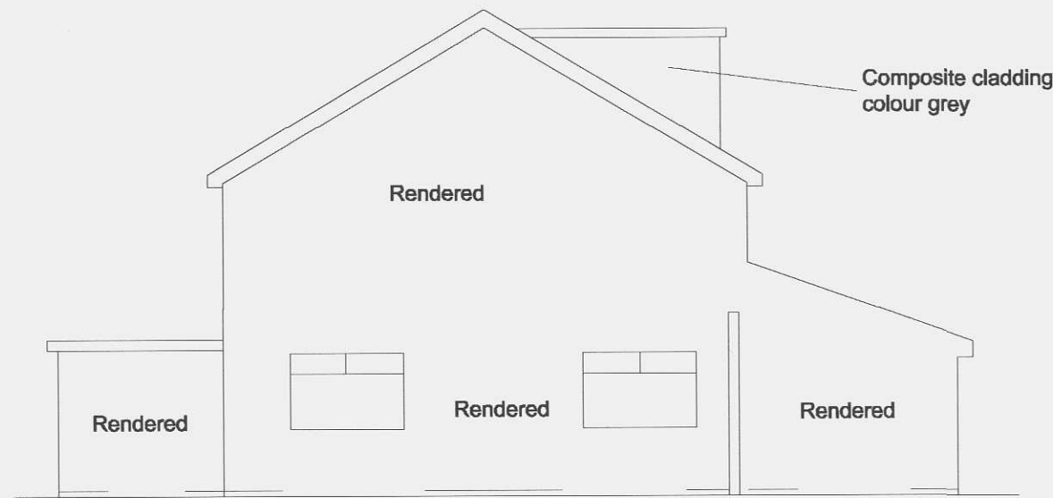
LEFT FLANK ELEVATION AS EXISTING
