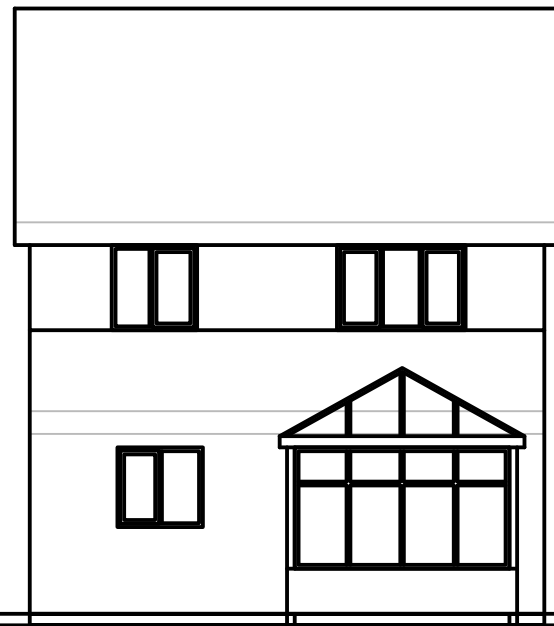
East elevation
