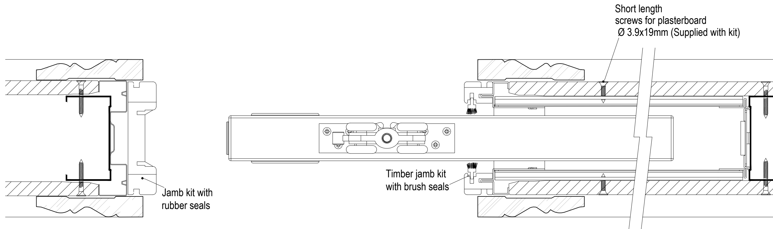
Internal Door Jamb Detail, scale 1:2
