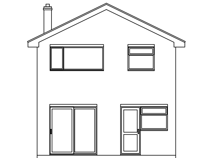
REAR ELEVATION
