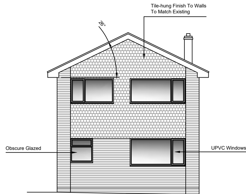
FRONT ELEVATION
