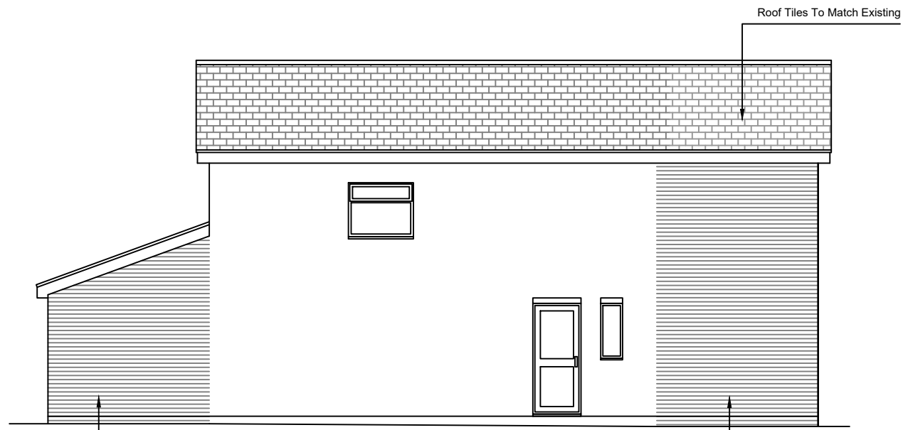
LEFT ELEVATION
