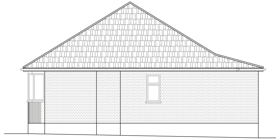
EXISTING SIDE ELEVATION-1
