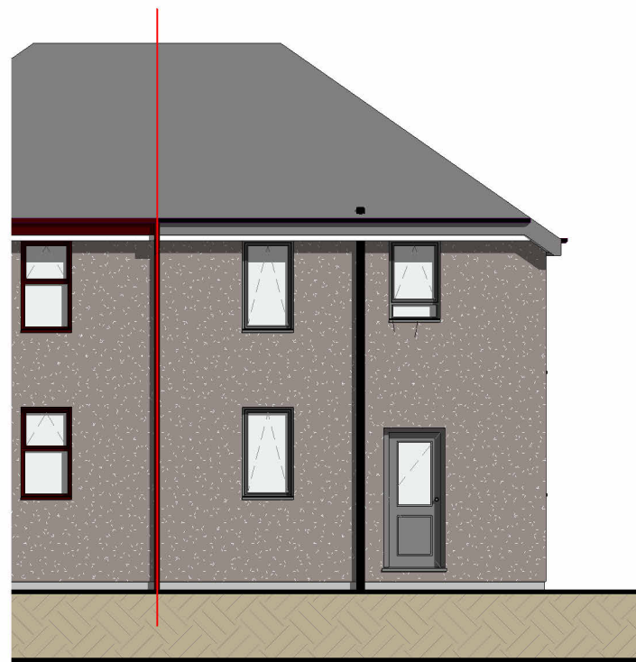
EX East Elevation
