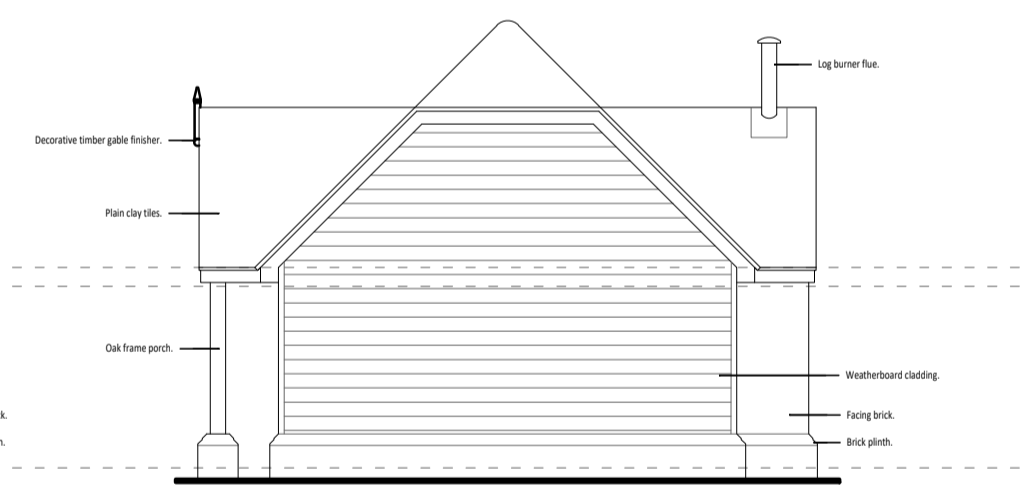
Plot 2 - Shelter shed - Side / East Elevation
