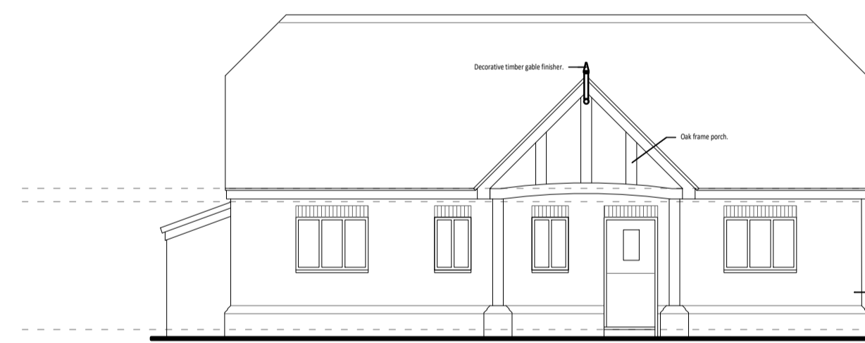
Plot 2 - Shelter shed - Front / South Elevation
