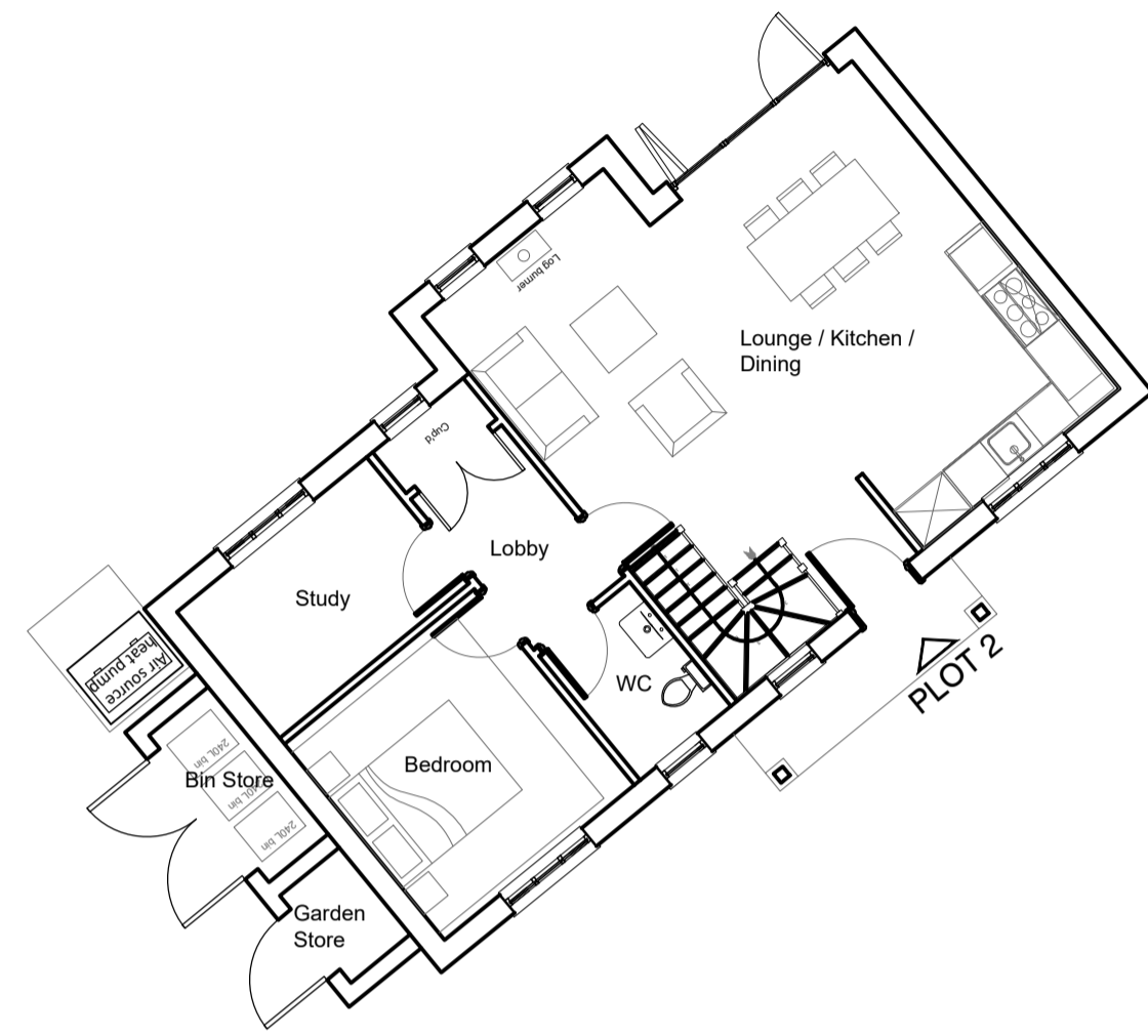
Ground floor
