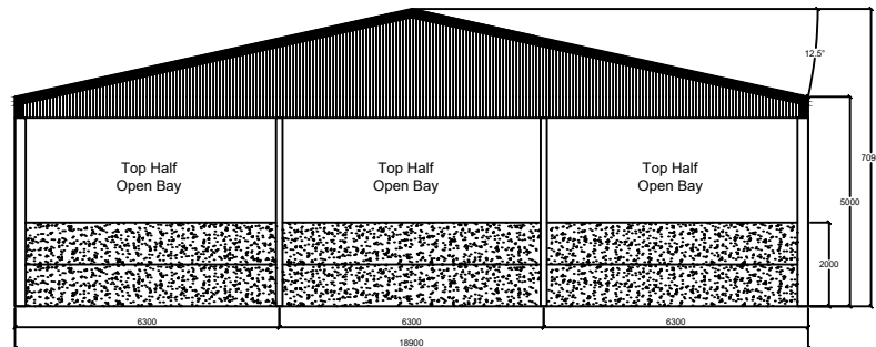
North Elevation
