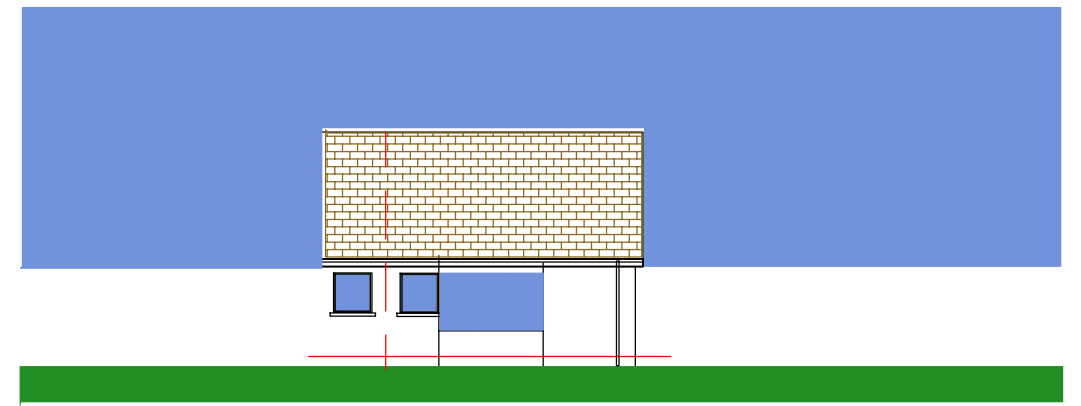
EXIST WEST ELEV @ 1:200 @ A3
