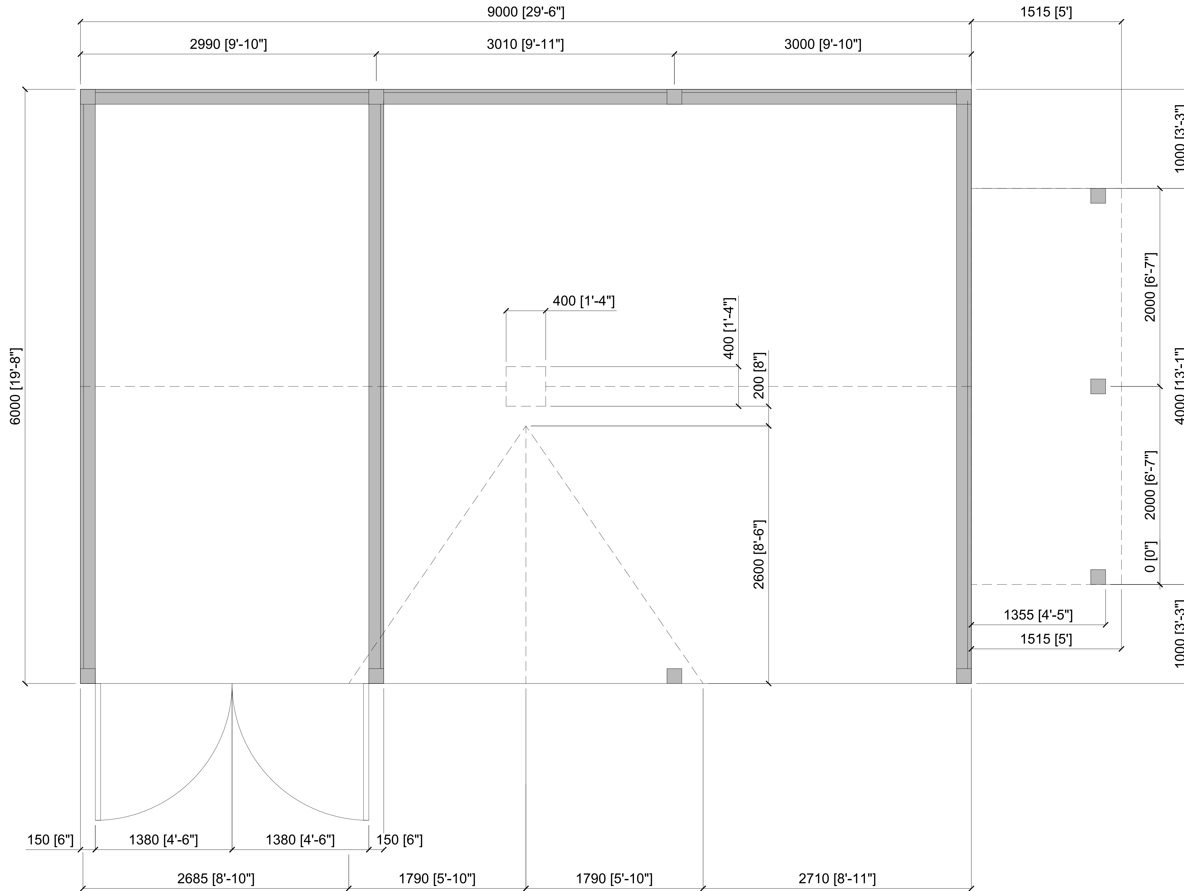
FLOOR PLAN
