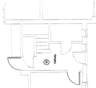
Ground floor plan 1:50
