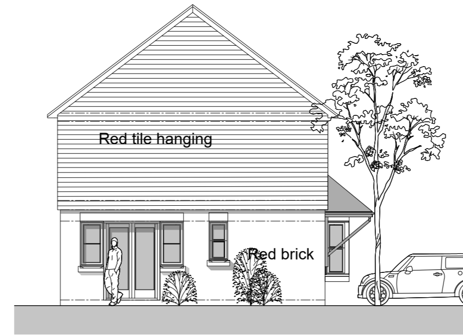
Proposed side elevation (west) 1:100
