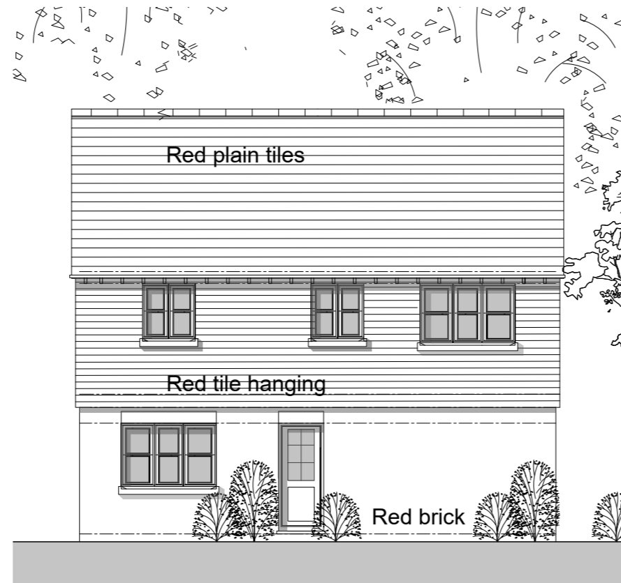
Proposed rear elevation (north) 1:100
