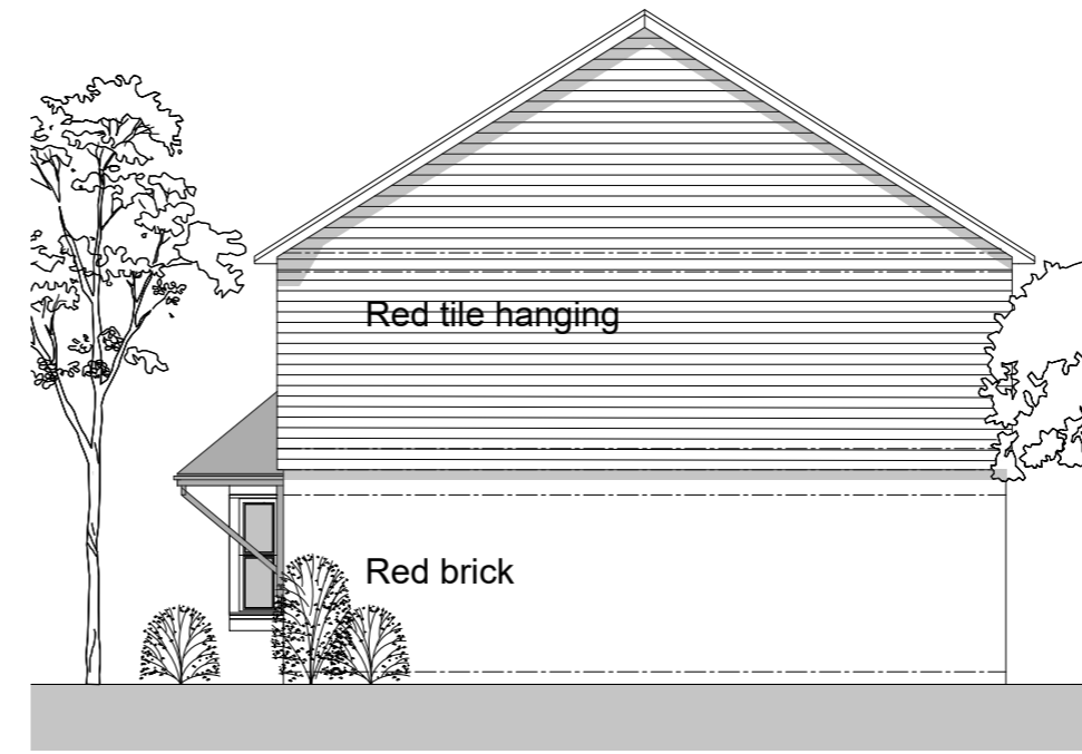
Proposed side elevation 1:100 Plot 1 South Plot 3 West
