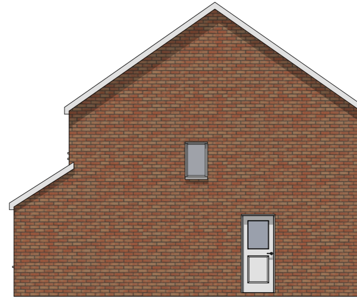
Existing Elevation - RH Side
