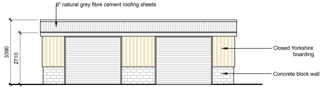
East Elevation 1 : 100
