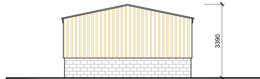
North Elevation 1 : 100
