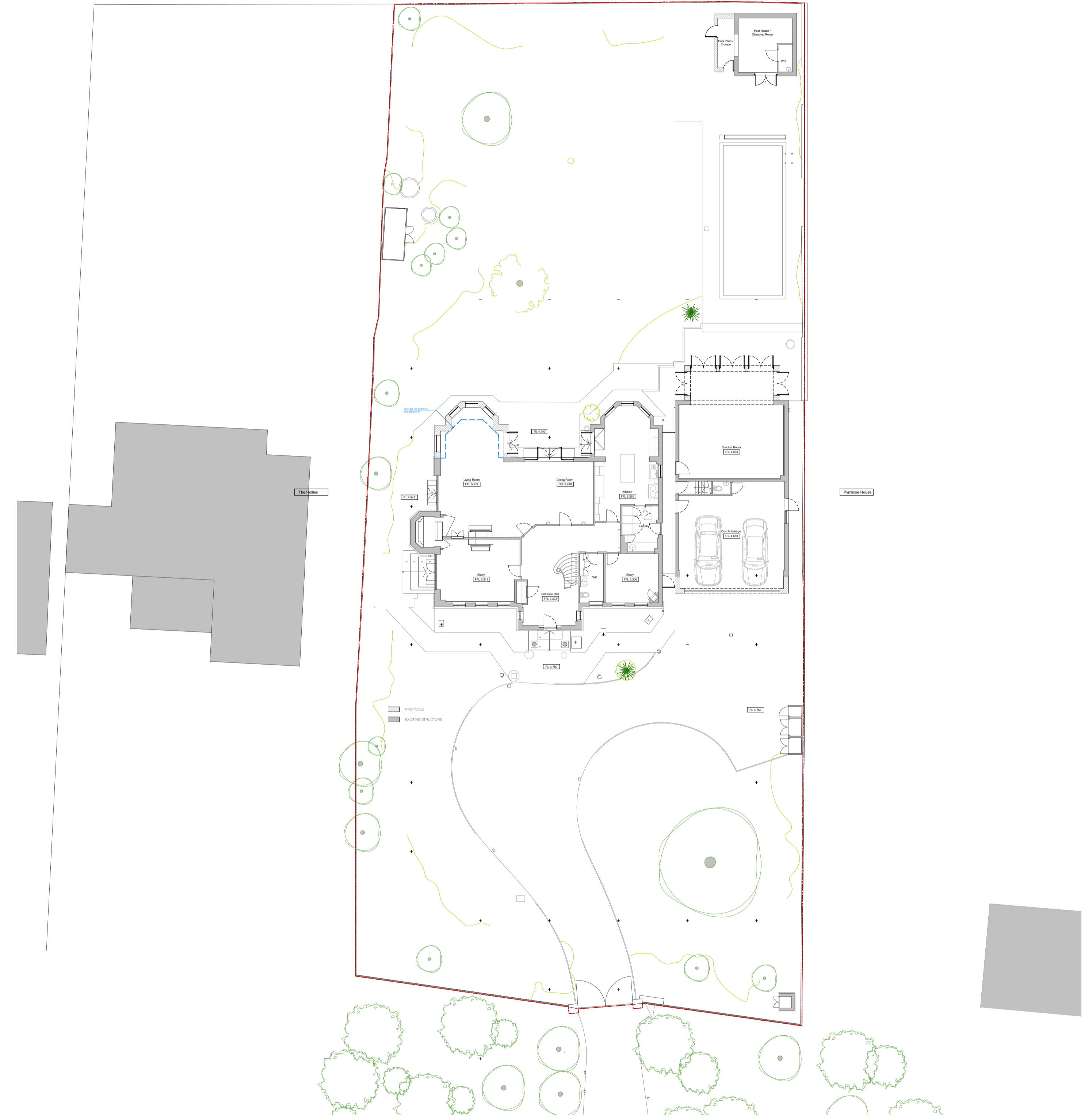
Proposed Site Layout Plan
