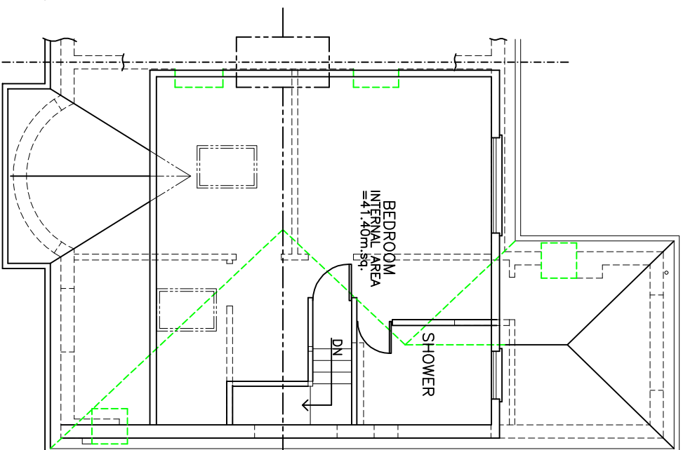
LOFT PLAN (1:100)
