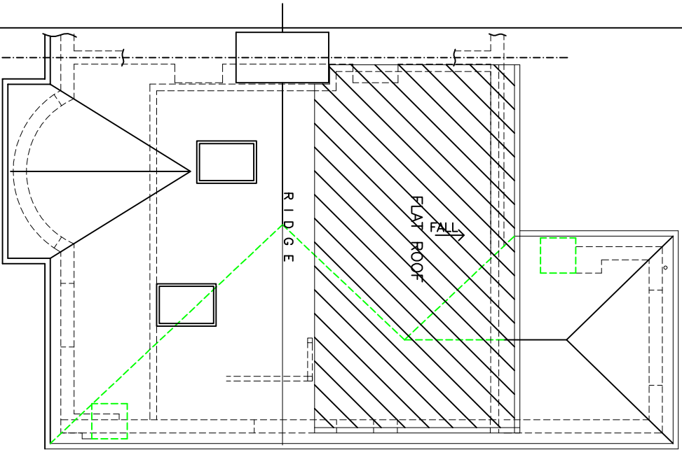
ROOF PLAN (1:100)
