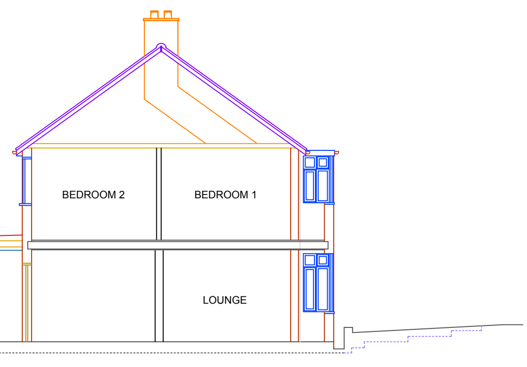
15 SECTION 'A-A' - PROPOSED 1:100
