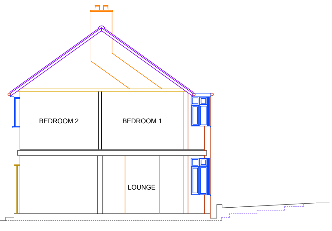
14 SECTION 'A-A' - EXISTING 1:100
