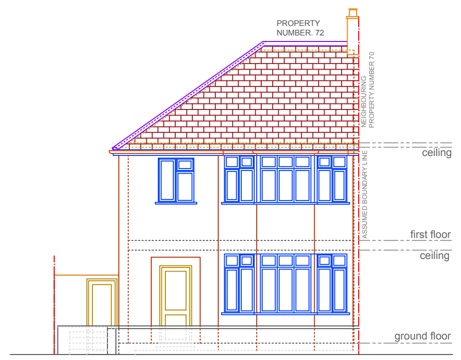
7 FRONT ELEVATION - EXISTING (NO CHANGES PROPOSED) 1:100
