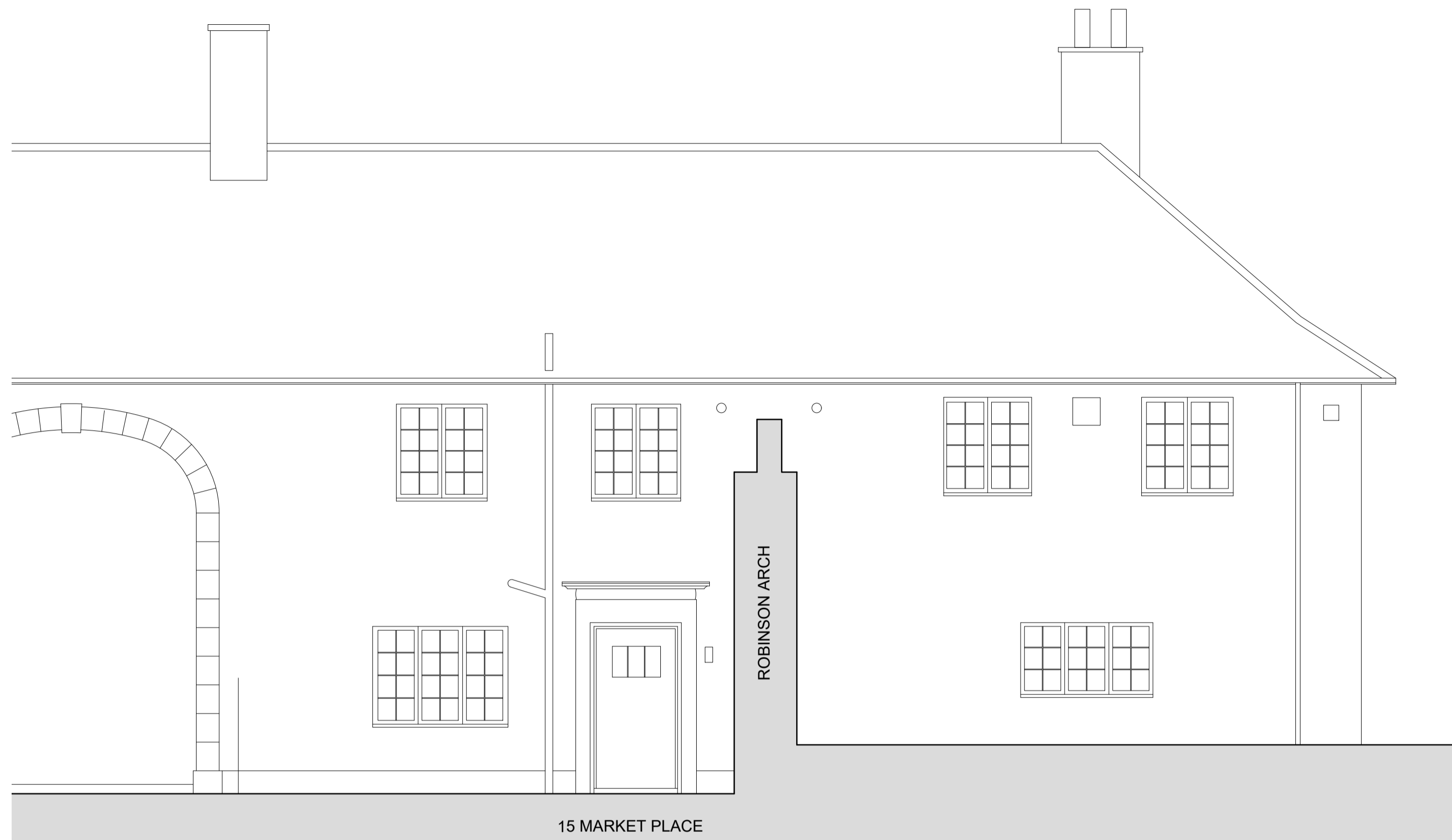
Front Elevation - Scale 1:100@A1
