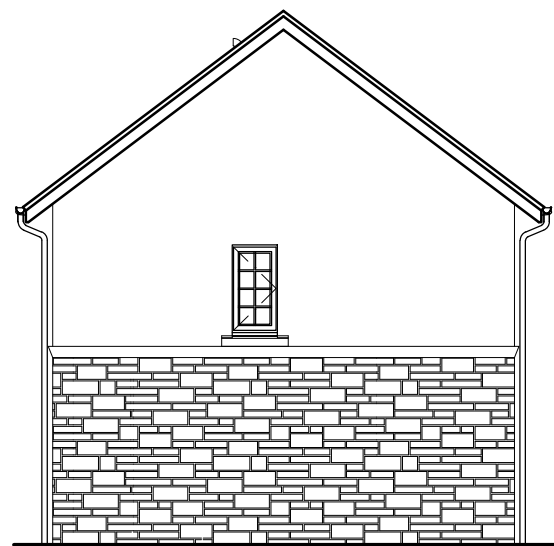
Rear Elevation
