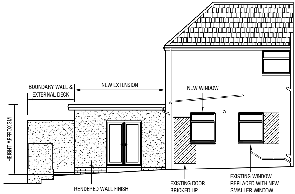
PROPOSED REAR SIDE ELEVATION
