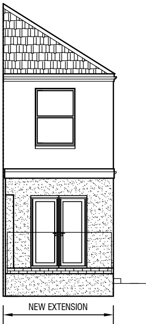
PROPOSED REAR ELEVATION
