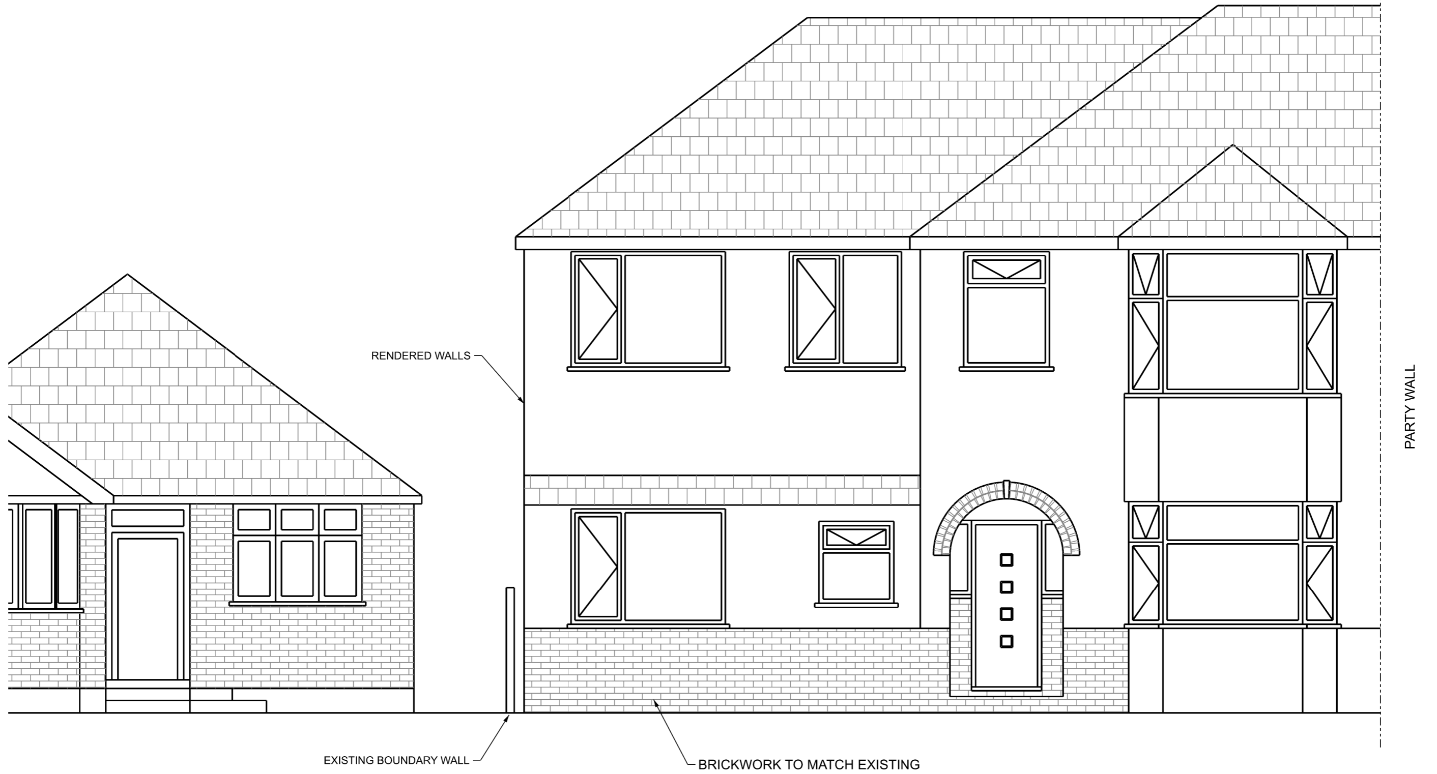
FRONT ELEVATION
