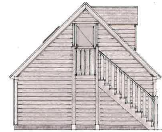
PROPOSED NORTH-EAST ELEVATION
