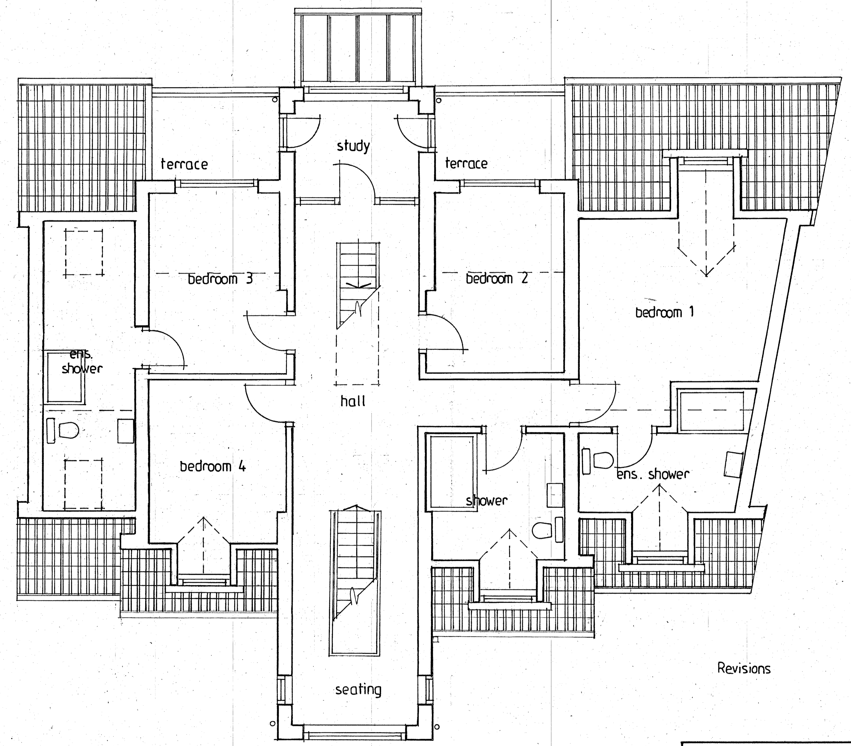
First Floor
