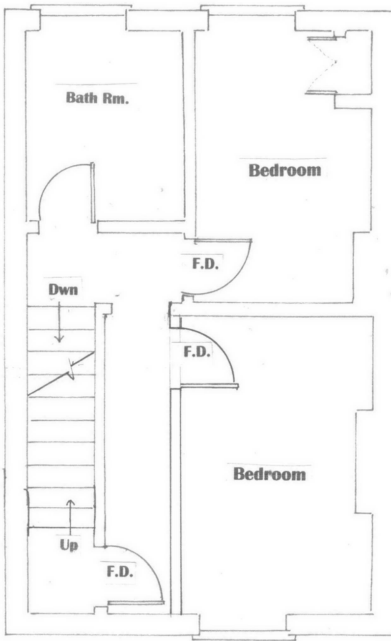
Proposed First Floor Layout 1 : 50 @ A 3
