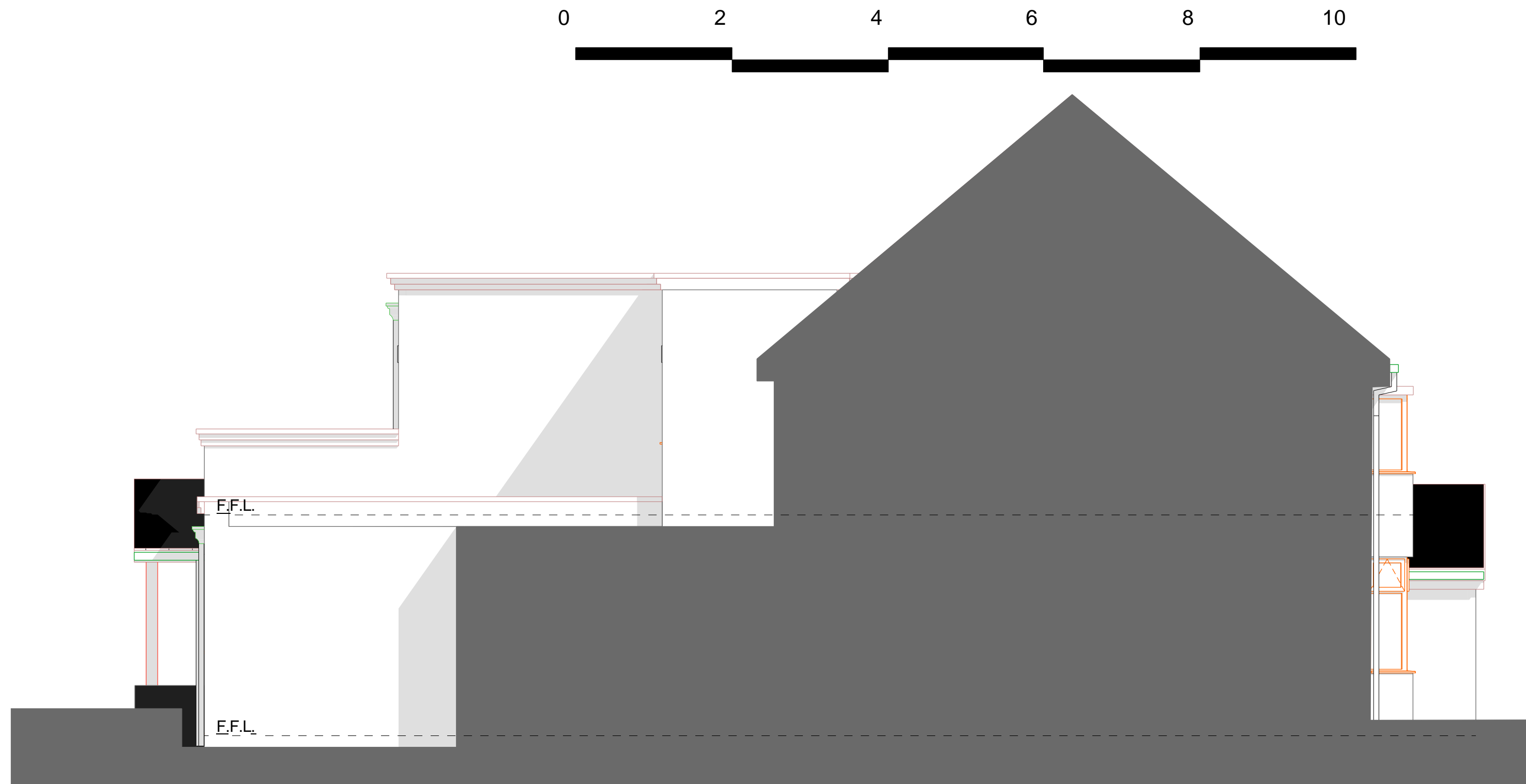
North Elevation (3)
