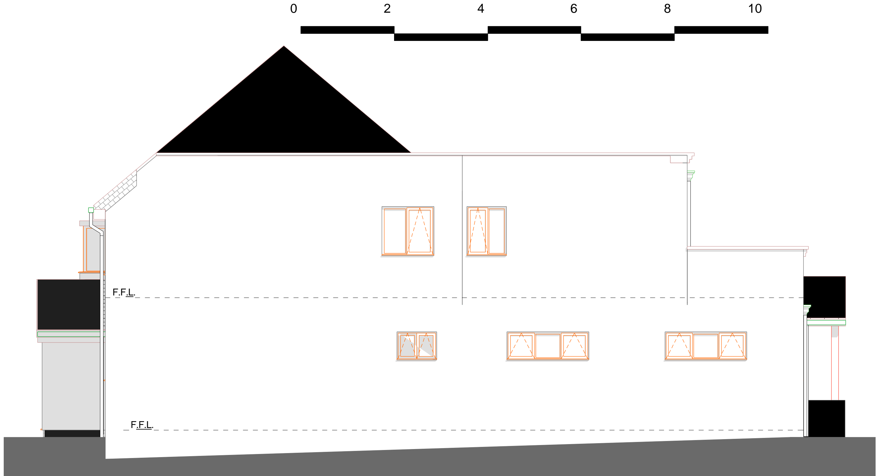
South Elevation (3)
