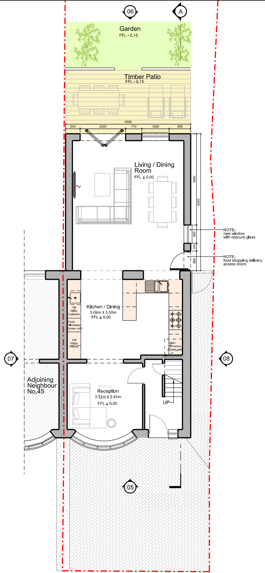
00 GROUND FLOOR PLAN 1:100
