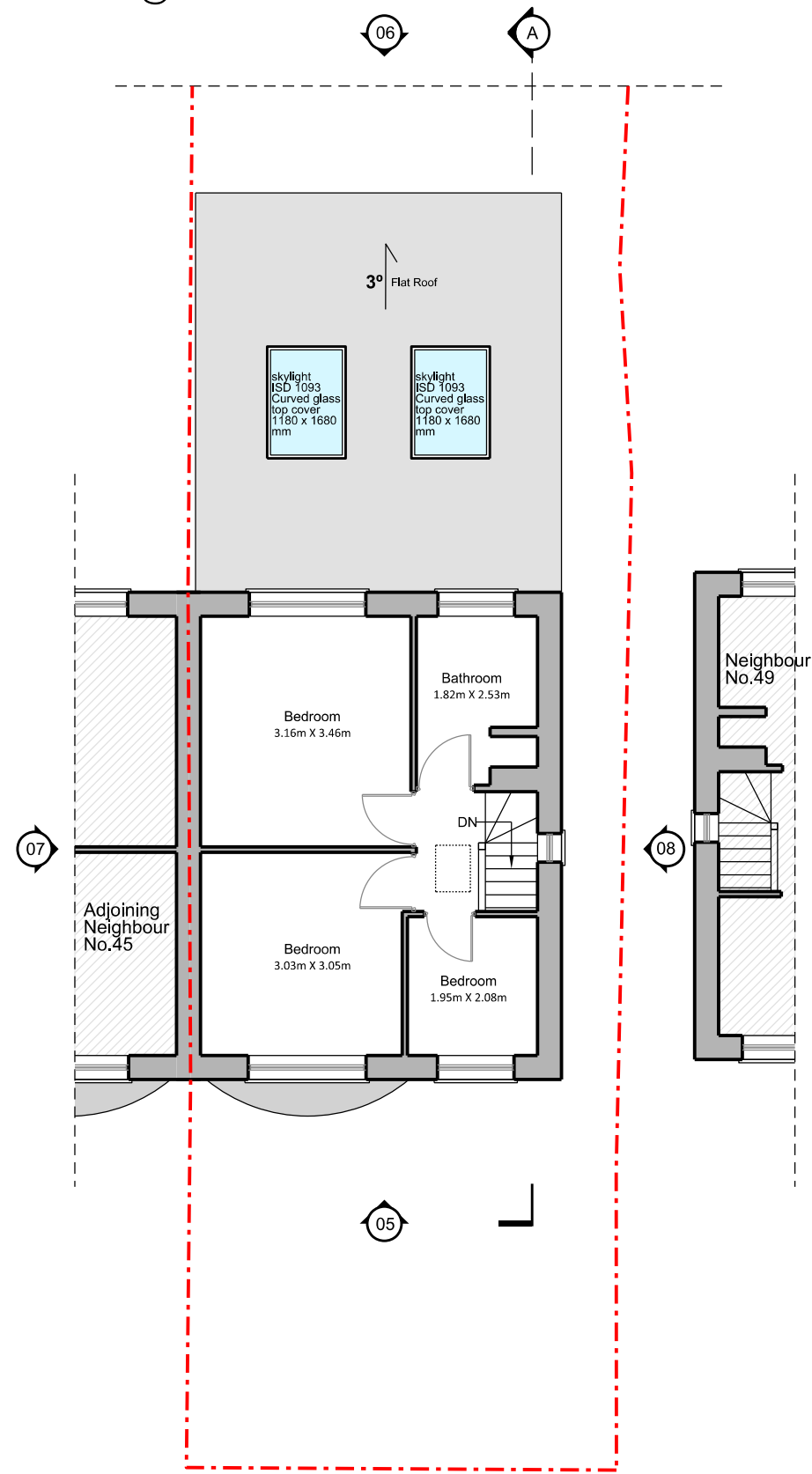
01 FIRST FLOOR PLAN 1:100
