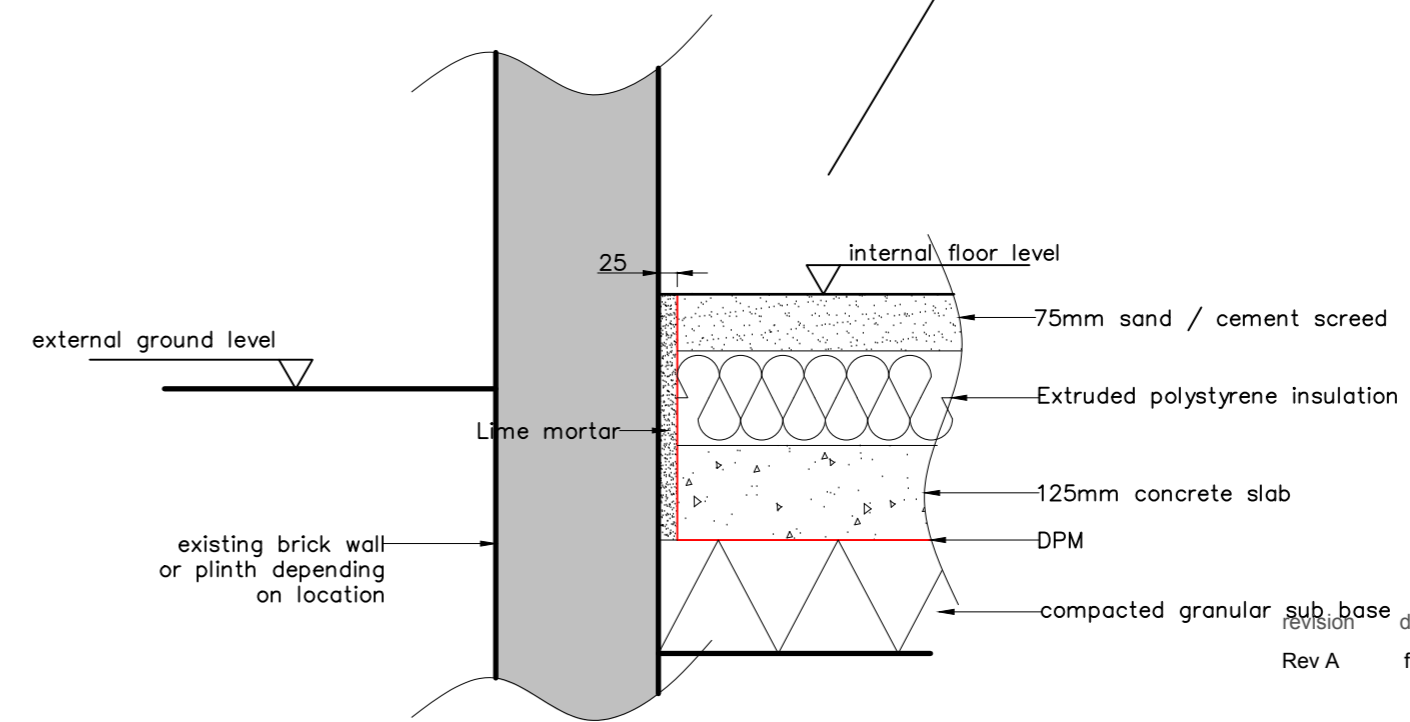
Detail through external wall / new floor scale 1:10
