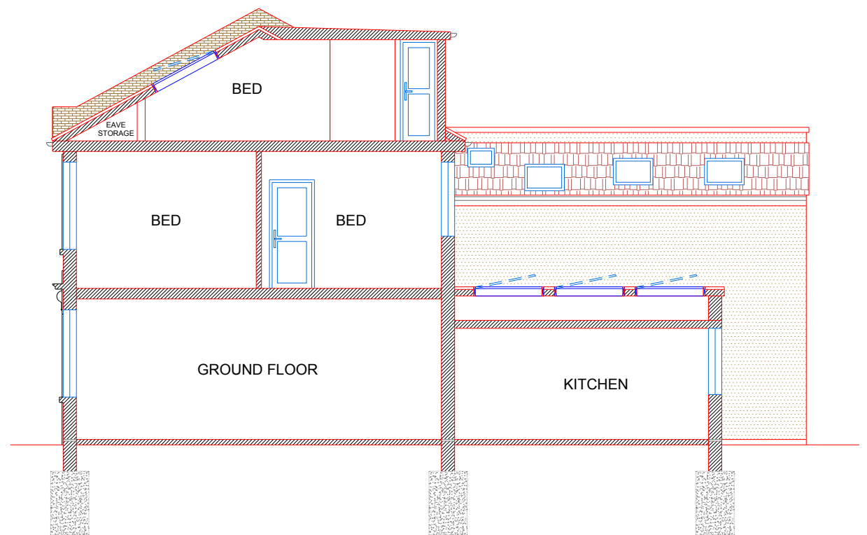
PROPOSED SECTION-AA
