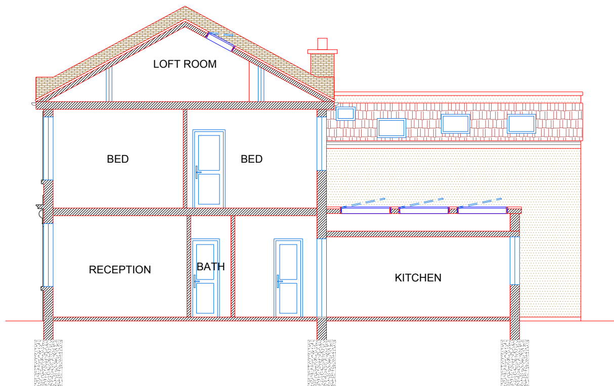
EXISTING SECTION-AA
