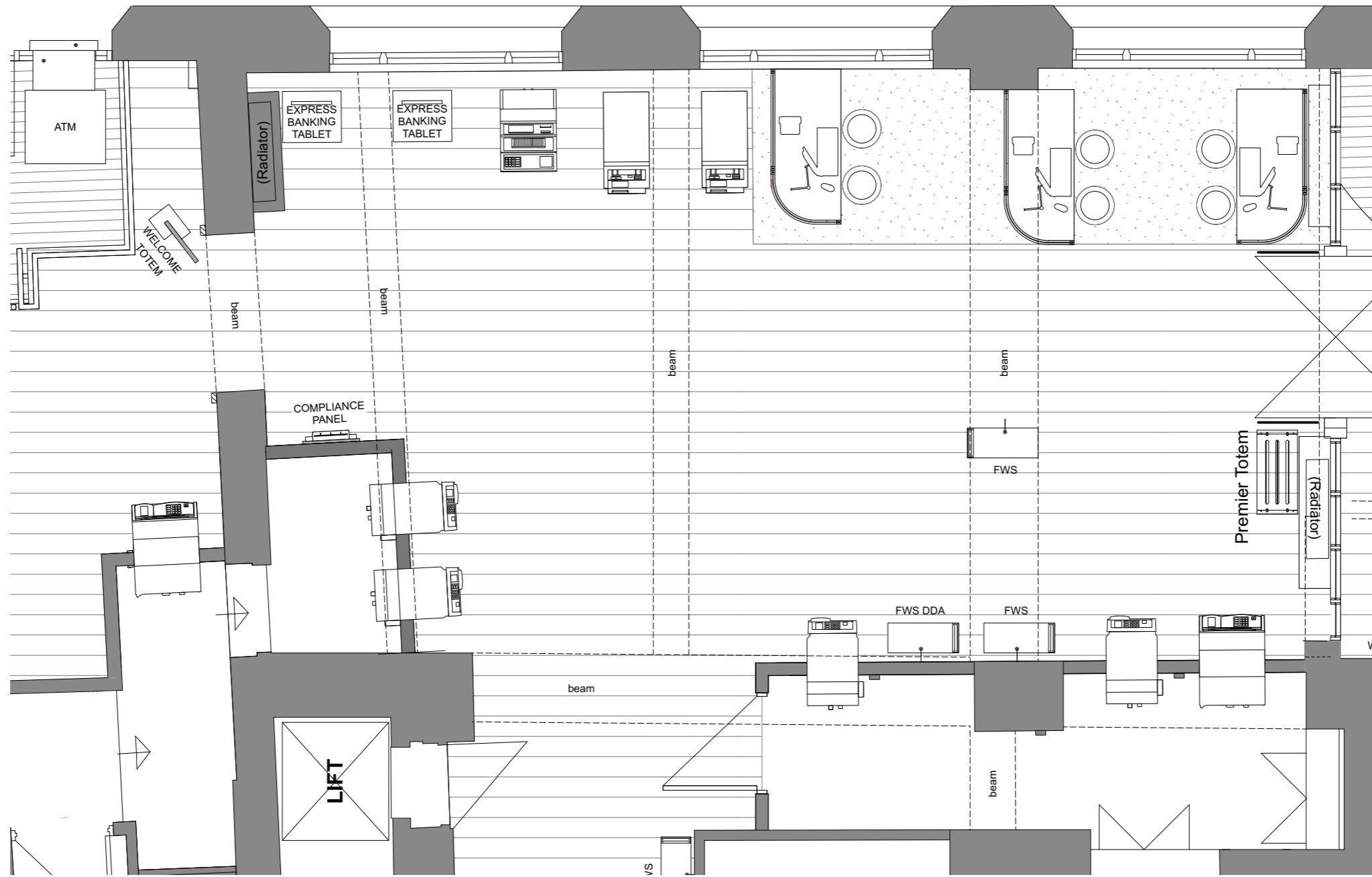
02 Plan of Affected Area 1:50@A3
