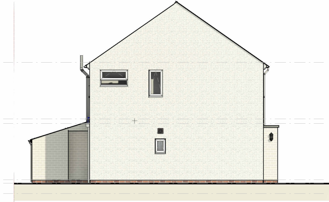
RS EX. RIGHTSIDE ELEVATION SCALE 1 : 100
