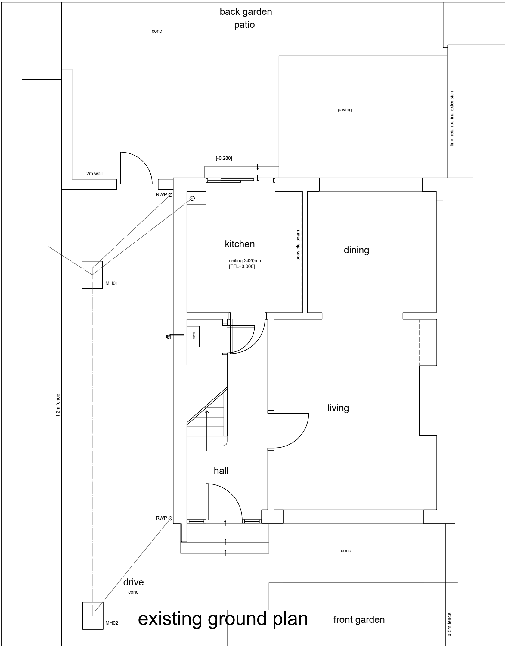
existing floor plan
