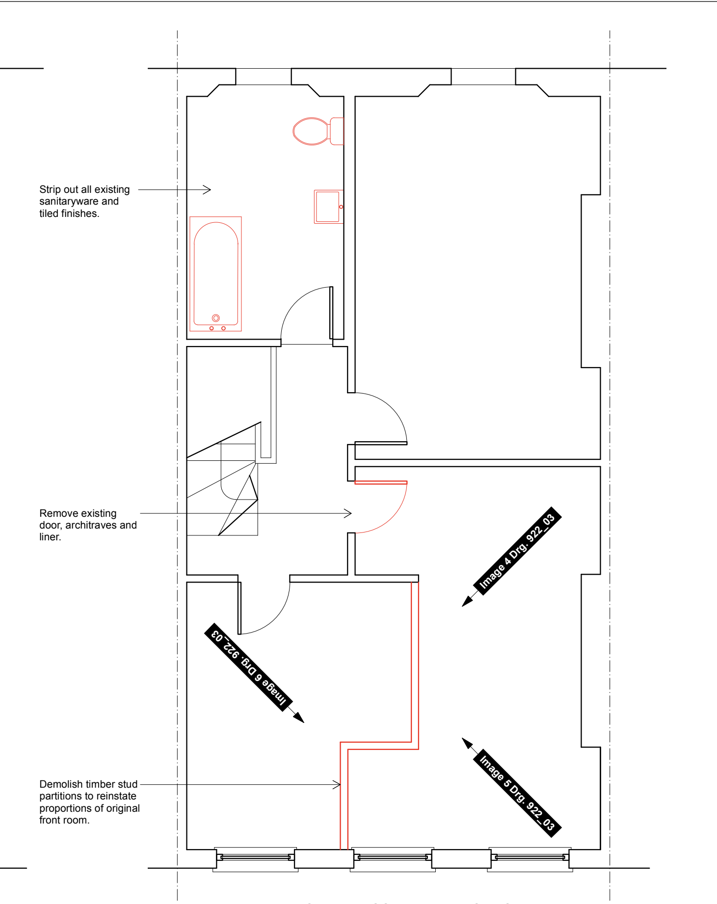
02_FOURTH FLOOR PLAN - EXISTING
