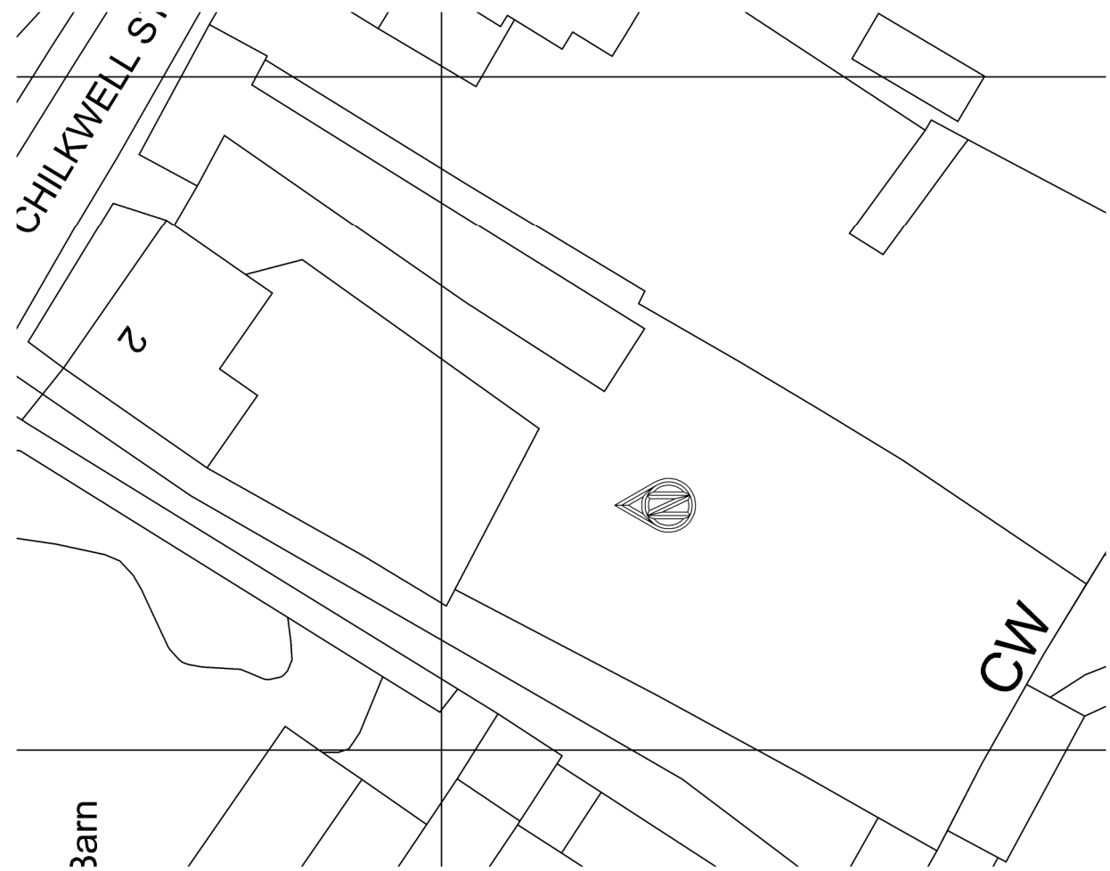
PROPOSED SITE/BLOCK PLAN Scale 1:500
