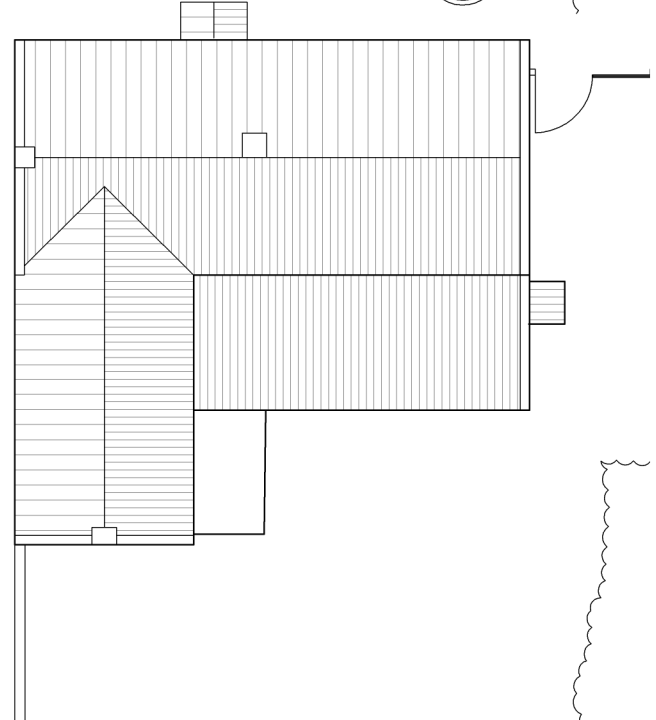
EXISTING ROOF PLAN Scale 1:200
