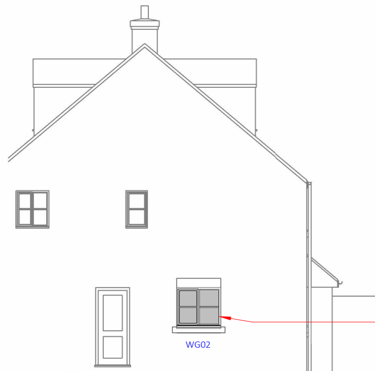
3 P03 west elevation - proposed 1 : 100
