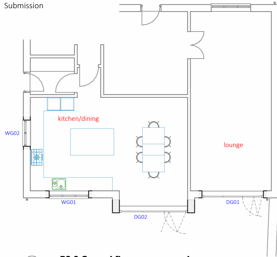
1 P03 P3.0 Ground floor as proposed 1 : 100
