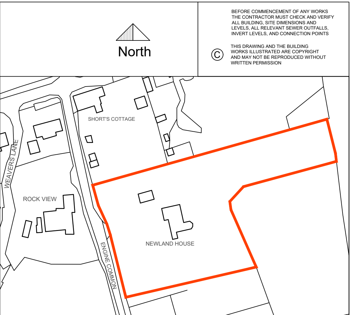
Area Plan Sc 1:1250
