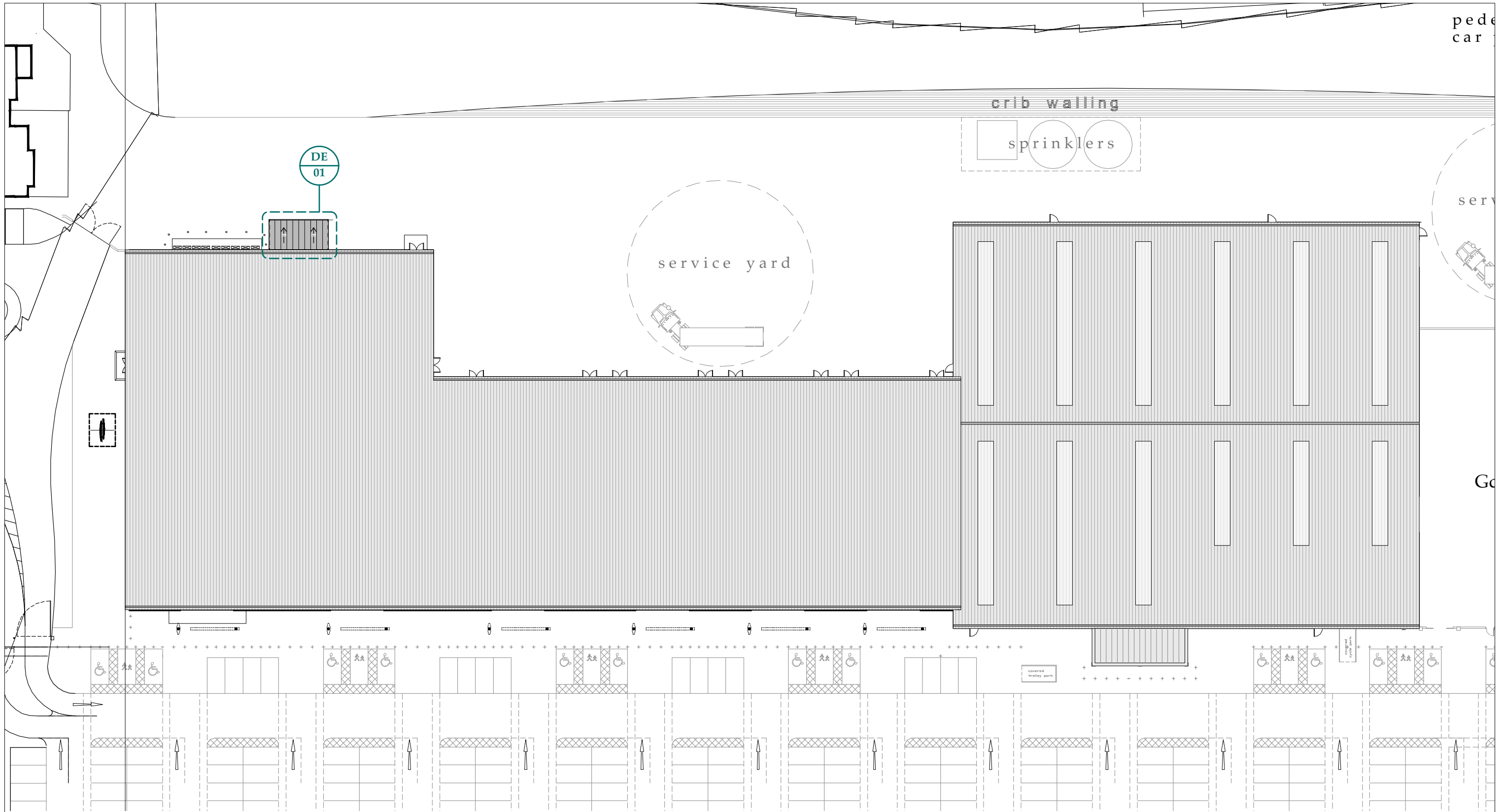
PROPOSED BLOCK PLAN | 1:500 @ A3
