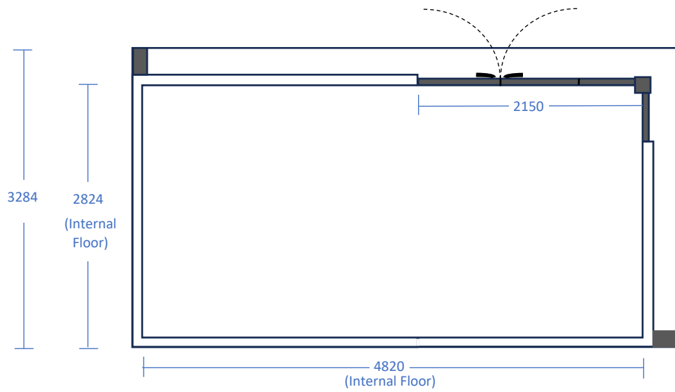
Floor Plan
